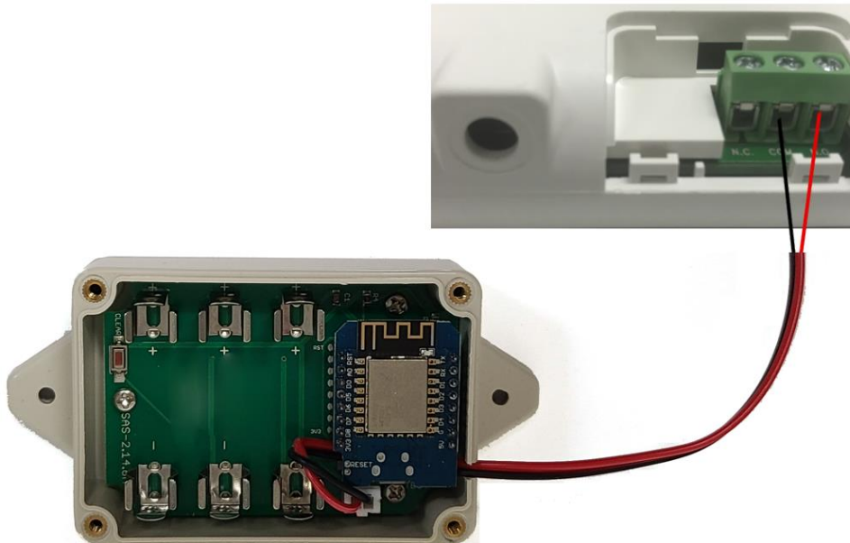
Optex RC20U Receiver Terminals (not to scale)
